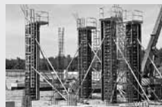
Column Formwork
